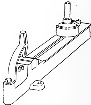
FIG. 176. SETTING STAKE FOR CIRCULAR SAWS.
